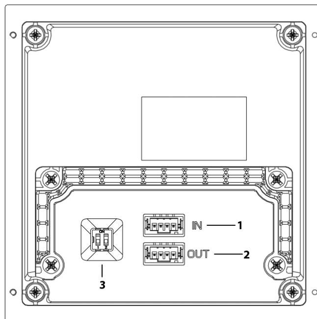
Figure 2-2 Rear panel of the 10-button module
